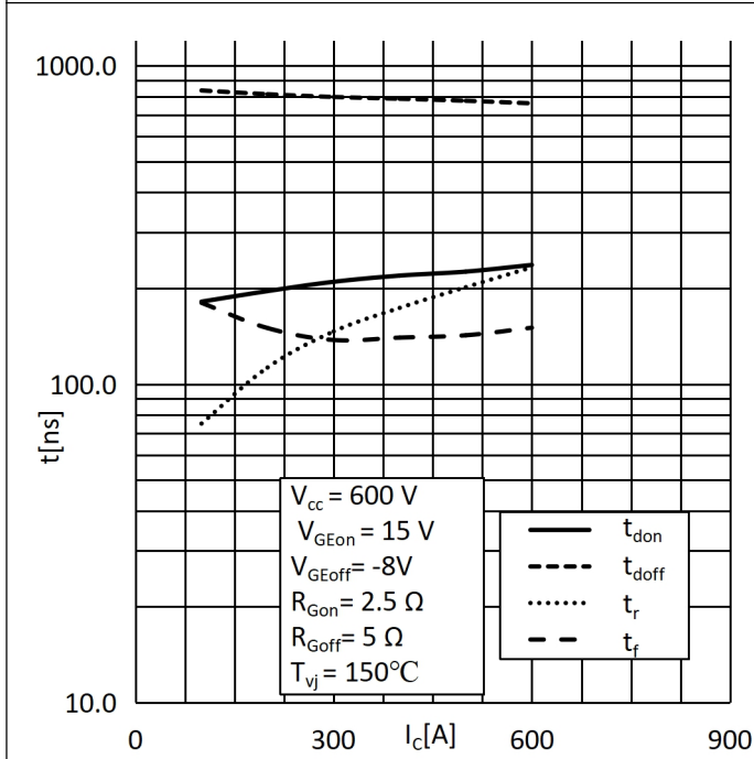
Fig.7: Switching Times vs. I_c
