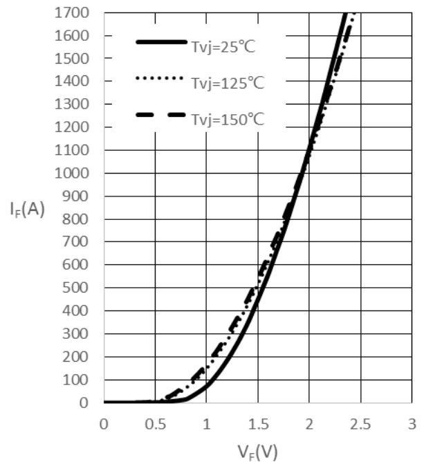
Fig.8: Forward characteristic
