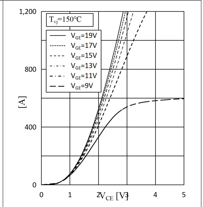
Fig.2: Output characteristics
