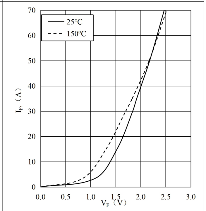
Fig.12 Typ. Forward Characteristics of Diode-Reverse 图 12 二极管正向偏压特性-反向恢复
