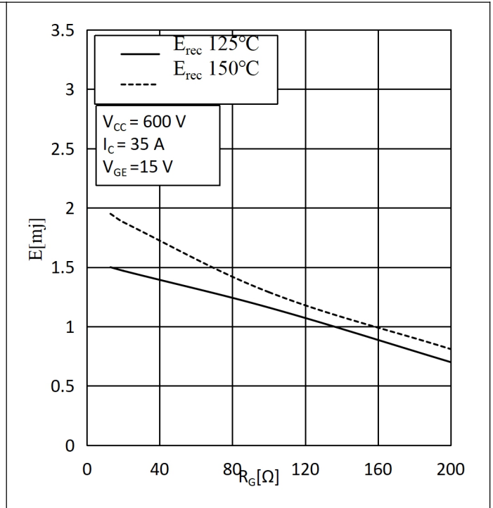
Fig.10: Reverse recovery Energy vs. Gate Resistor-Reverse 图 10: 反向恢复损耗与门极电阻关系-反向恢复
