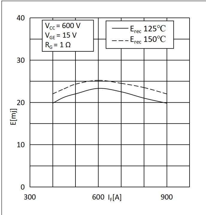
Fig.9: Reverse recovery Energy-Chopper 图 9: 反向恢复损耗-斩波
