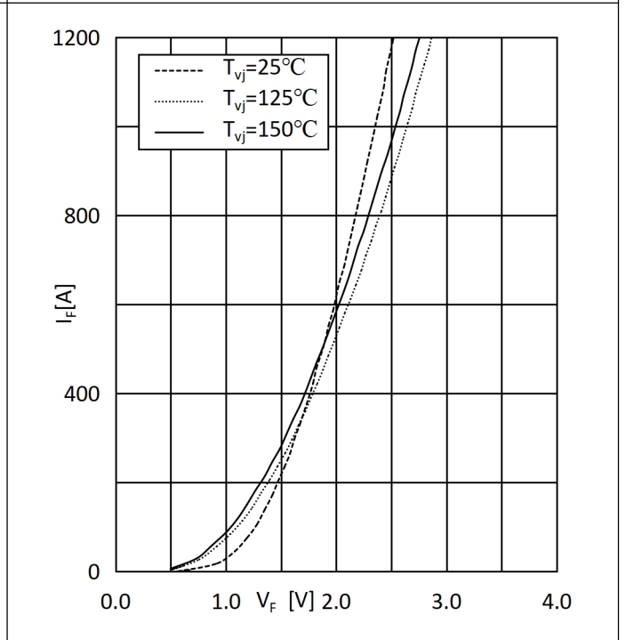
Fig.8: Forward characteristic-Chopper
