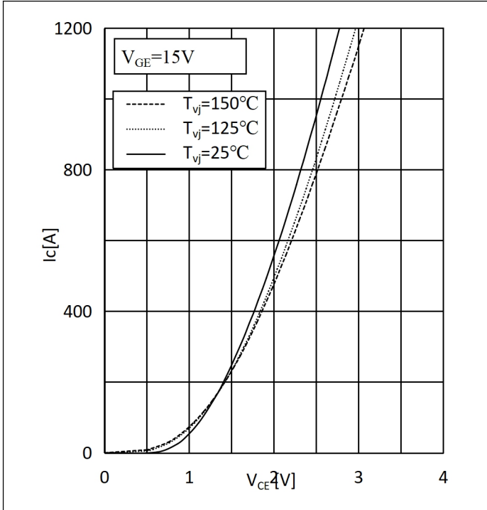
Fig.1: Output Characteristics
