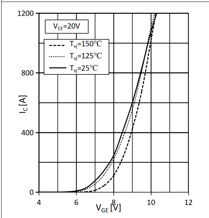
Fig.3: Transfer Characteristics
