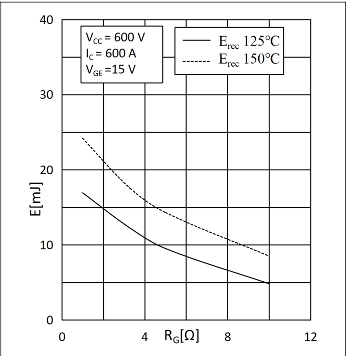
Fig.10: Reverse recovery Energy vs. Gate Resistor
