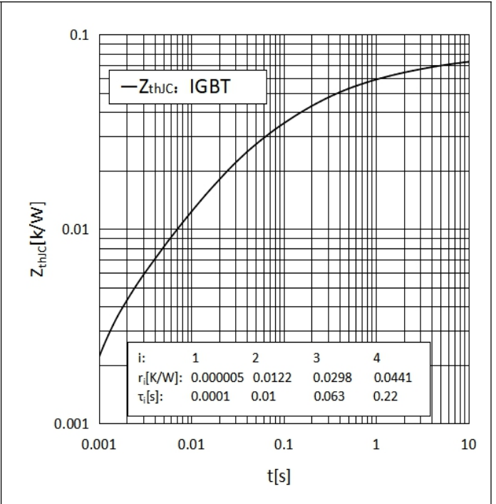
Fig.14: Typ. transient thermal impedance
