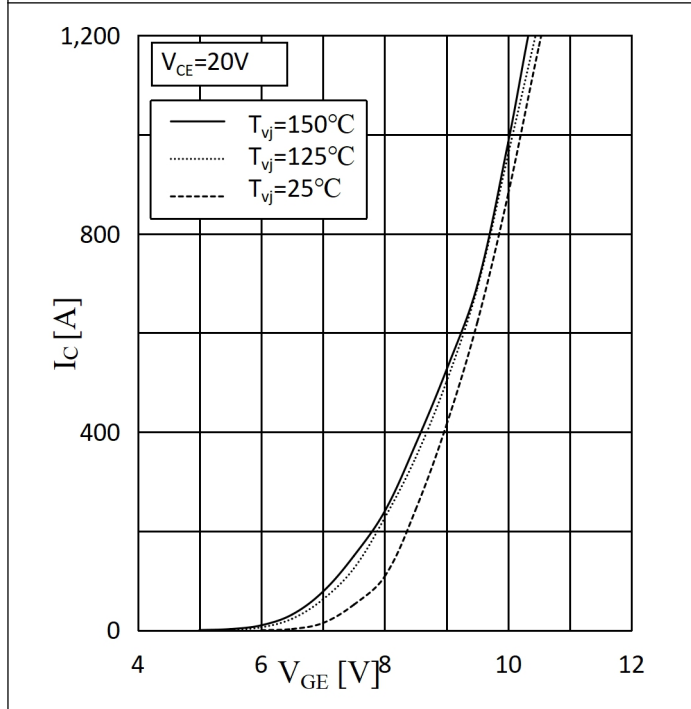
Fig.3: Transfer Characteristics
