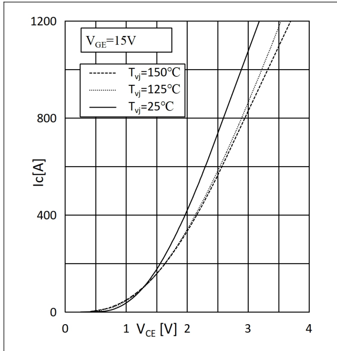
Fig.1: Output Characteristics
