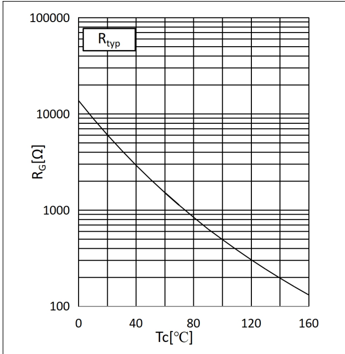
Fig.13:Typ. NTC-Temperature Characteristics
