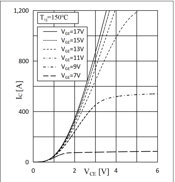
Fig.2: Output characteristics
