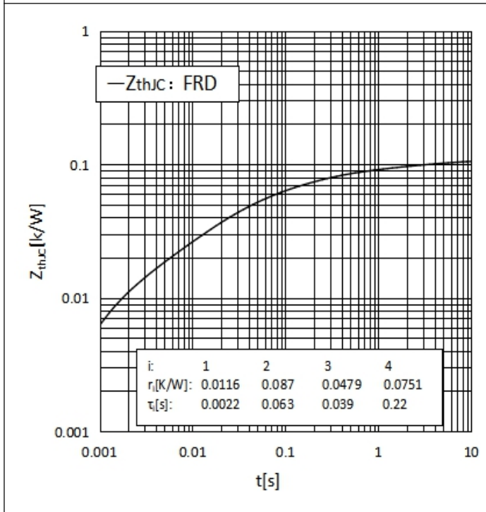
Fig.15: Typ. transient thermal impedance
