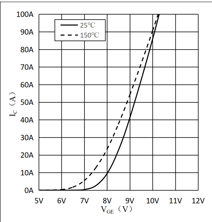
Fig.2 Typ. Transfer Characteristics-Inverter
