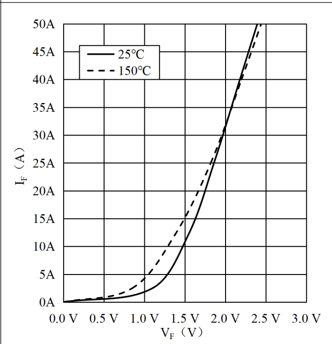
Fig. 12 Forward Characteristics of Diode- Brake-Chopper
