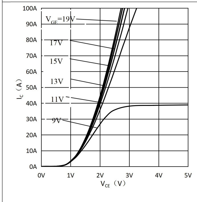
Fig.3 Typ. Output Characteristics-Inverter
