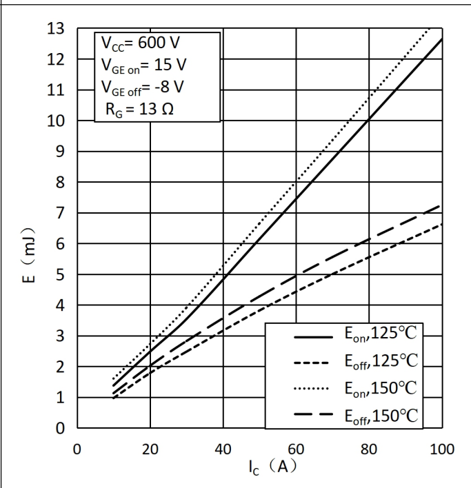
Fig.4 Switching Loss vs. Collector Current-Inverter
