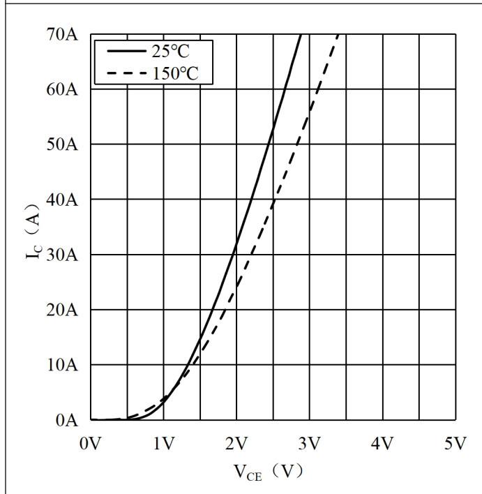
Fig.11 Typ. Output Characteristics, Brake-Chopper
