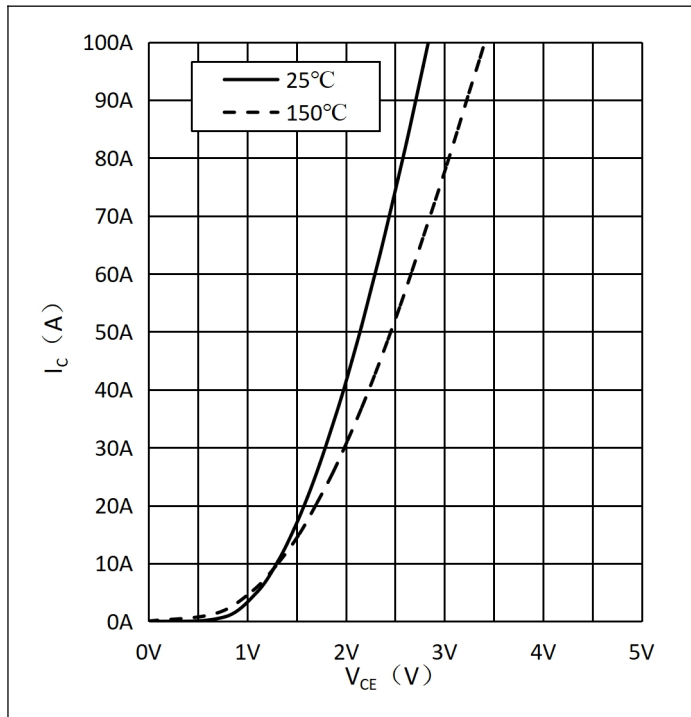
Fig.1 Typ. Output Characteristics-Inverter
