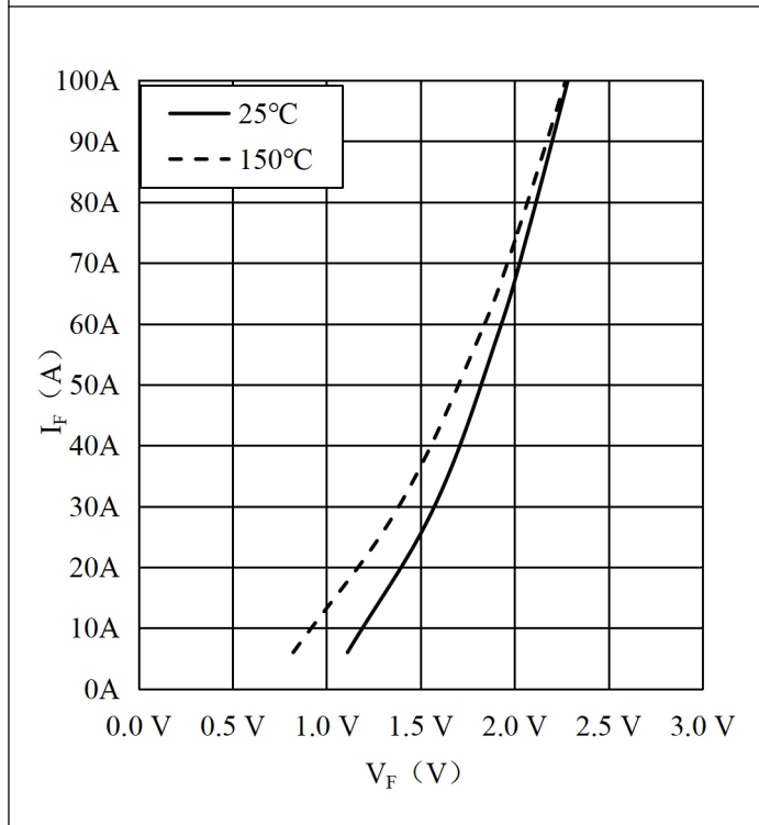
Fig.7 Typ. Forward Characteristics of Diode-Inverter 图 7 二极管正向偏压特性-逆变器
