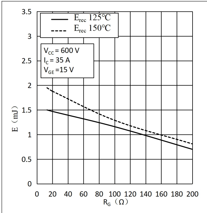
Fig.9 Switching Loss of Diode vs. Gate Resistor -Inverter 图 9 FRD 开关损耗和门极电阻-逆变器
