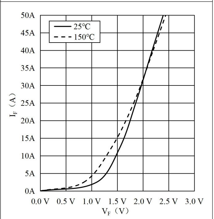
Fig.12 Forward Characteristics of Diode- Brake-Chopper 图 12 二极管正向偏压特性, 制动-斩波器
