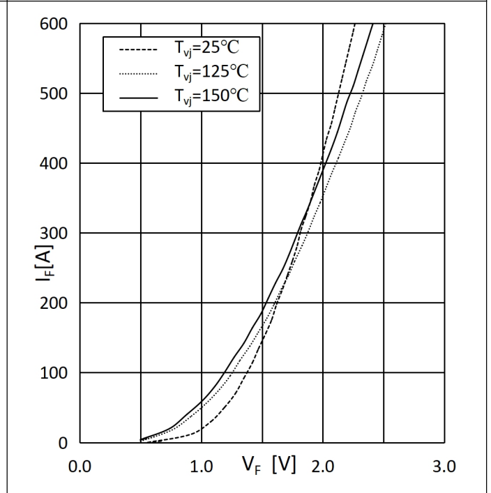
Fig.8: Forward characteristic-Chopper
